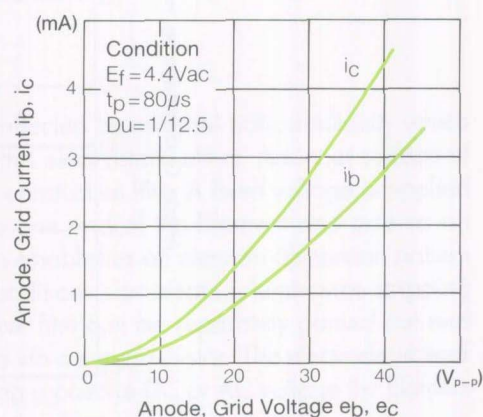
Figure 18. e_b, e_c - i_b, i_c Characteristics (Dynamic Drive)
