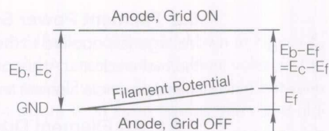
Figure 14. Relation of Electrode Potentials in Case of Figure 13
