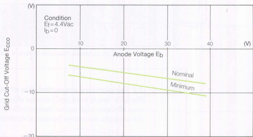
Figure 22. E_b - E_{c0} Characteristics (One End of the Filament Grounded)
