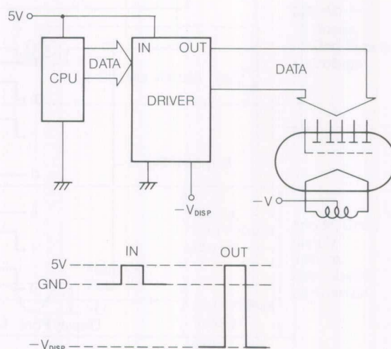
Figure 31. Typical Drive Circuit (Negative power supply use, Parallel-in-Parallel-out)
