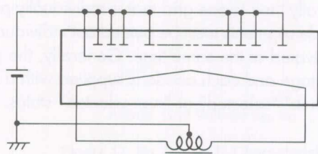
Figure 11. Basic Connection Diagram for Alternating Current as the Filament Voltage (2) (Center Tap of the Filament Transformer Grounded)
