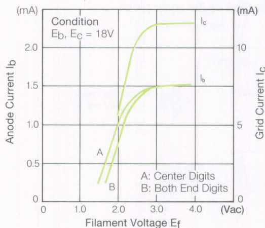
Figure 7. E_f - I_b, I_c Characteristics
