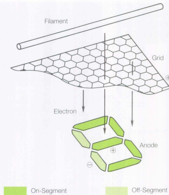
Figure 3. Principle of VFD Operation
